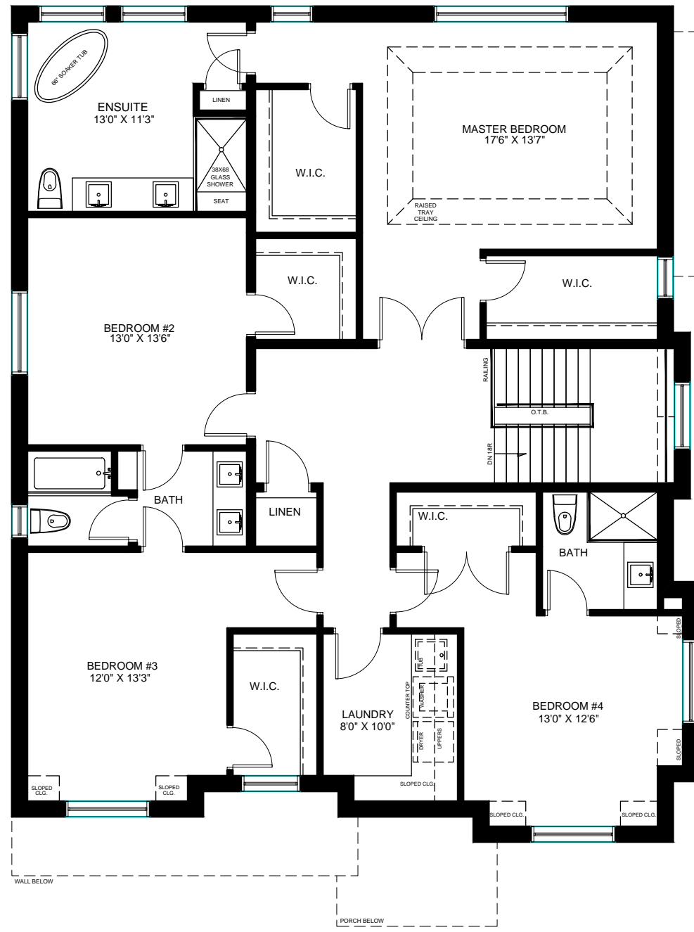
SECOND FLOOR PLAN SCALE: AS NOTED ON PAGE
