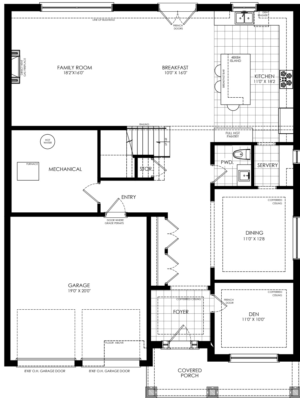
PROPOSED GROUND FLOOR PLAN 'A' SCALE: AS NOTED ON PAGE (LOT 8 & 9)
