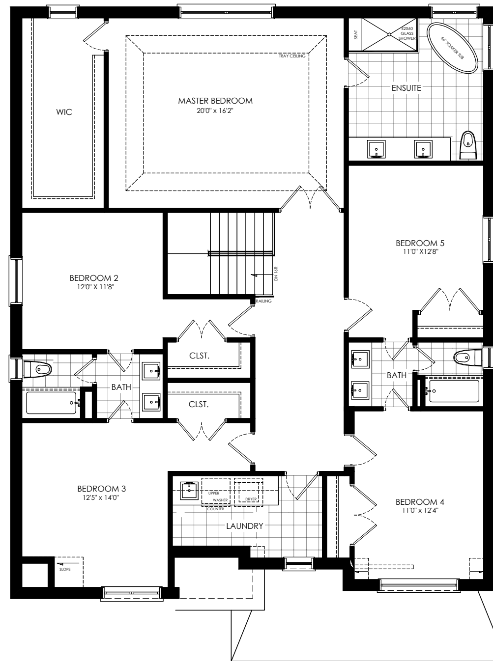
PROPOSED SECOND FLOOR PLAN 'A' SCALE: AS NOTED ON PAGE (LOT 8 & 9)
