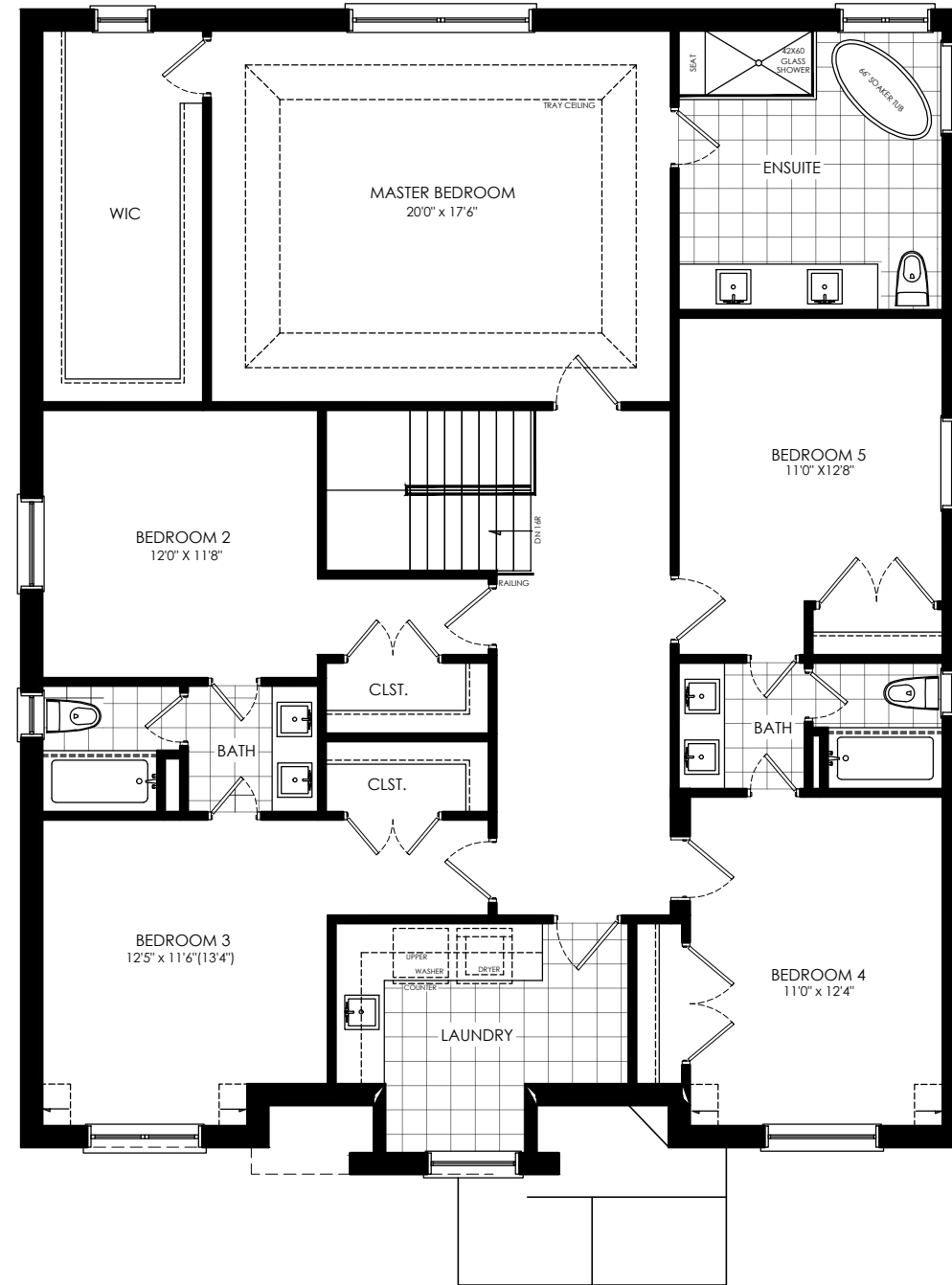
PROPOSED SECOND FLOOR PLAN 'B' SCALE: AS NOTED ON PAGE (LOT 8 & 9)
